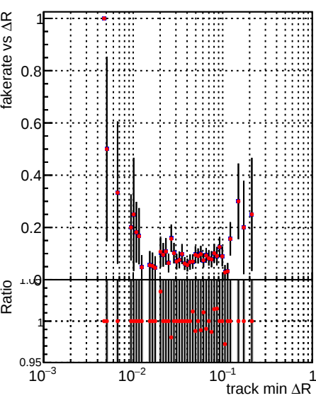
Legend: DQM_TT_ORIGINAL (black line with error bars), DQM_TT_MODIFIED_layerProcV2_PRVersion (red line with error bars)
