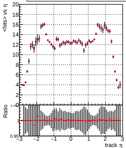
mean hits vs \eta Legend: DQM_TT_ORIGINAL (blue line), DQM_TT_MODIFIED_layerProcV2_PRVersion (red line)
