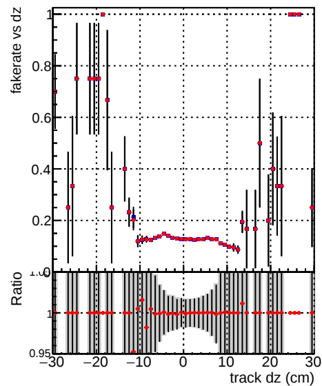
Fake rate vs dz Legend: —•— DQM TT ORIGINAL —•— DQM TT MODIFIED_layerProcV2_PRVersion
