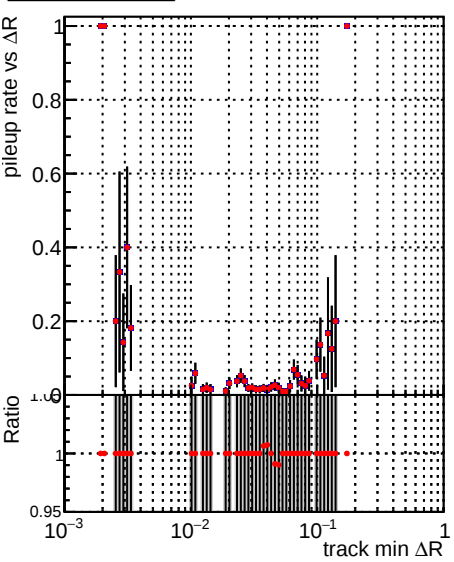
Legend: DQM_TT_ORIGINAL (grey bars), DQM_TT_MODIFIED_layerProcV2_PRVersion (red dots)
