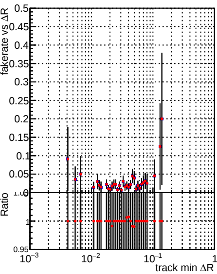
Legend: DQM_TT_ORIGINAL (grey bars), DQM_TT_MODIFIED_layerProcV2_PRVersion (red dots)
