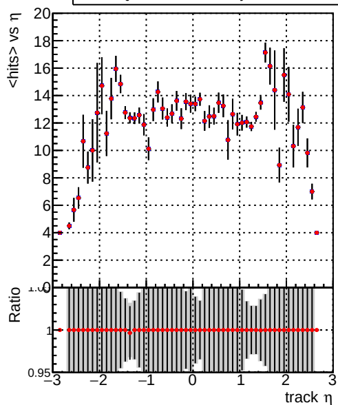
mean hits vs \eta Legend: DQM_TT_ORIGINAL (blue line with error bars), DQM_TT_MODIFIED_layerProcV2_PRVersion (red line with error bars)
