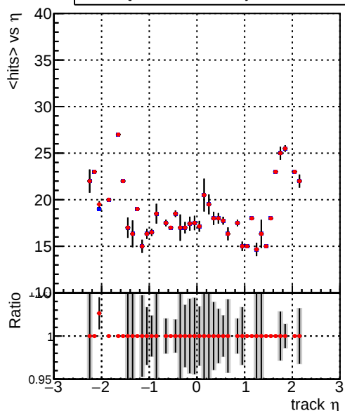
mean hits vs \eta Legend: DQM_TT_ORIGINAL (blue line with dots), DQM_TT_MODIFIED_layerProcV2_PRVersion (red line with dots)
