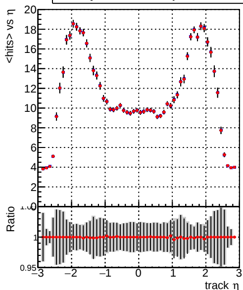
mean hits — DQM_TT_ORIGINAL — DQM_TT_MODIFIED_layerProcV2_PRVersion
