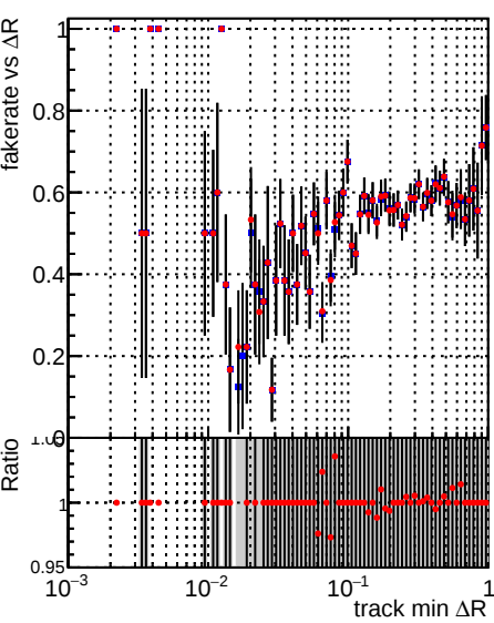
Legend: DQM_TT_ORIGINAL (grey bars with blue error bars), DQM_TT_MODIFIED_layerProcV2_PRVersion (red dots with error bars)
