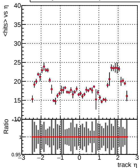
mean hit Legend: DQM_TT_ORIGINAL (blue line), DQM_TT_MODIFIED_layerProcV2_PRVersion (red line)
