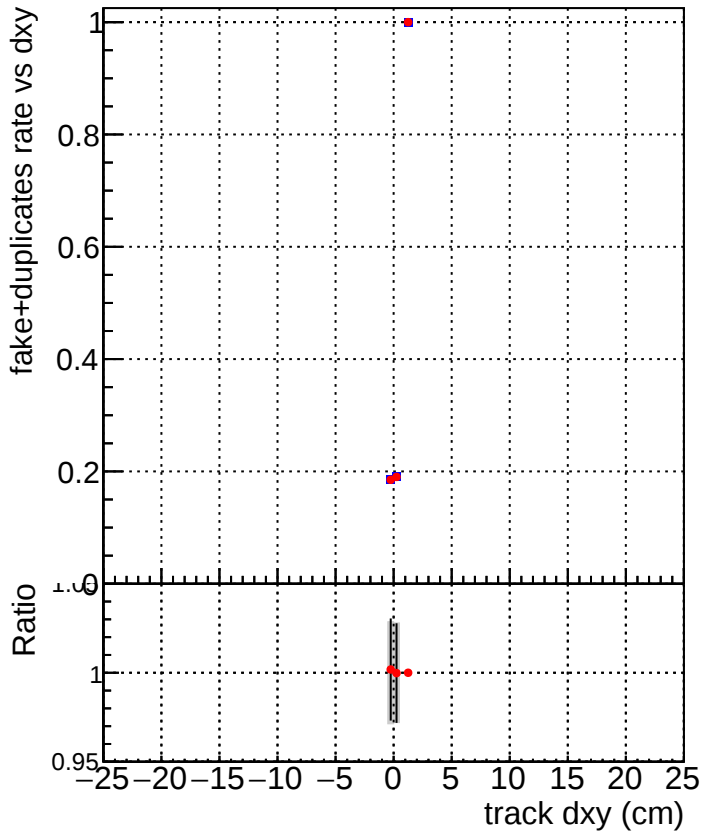
Legend: DQM_TT__ORIGINAL (grey square) DQM_TT__MODIFIED_layerProcv2_PRVersion (red circle)
