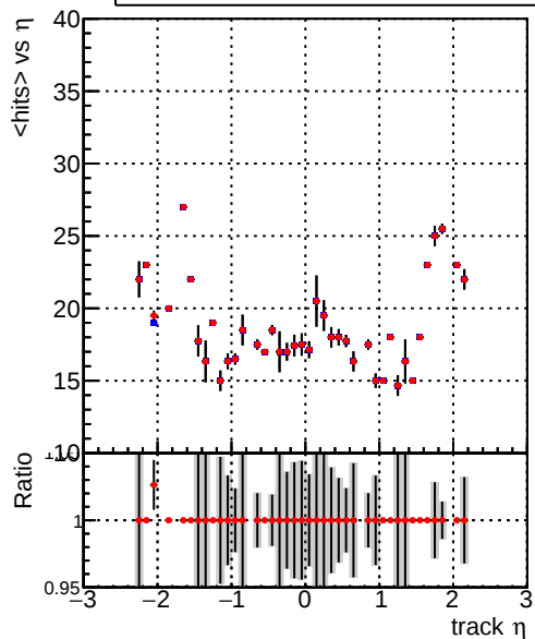
mean hit Legend: DQM_TT_ORIGINAL (blue line with dots), DQM_TT_MODIFIED_layerProcv2_PRVersion (red line with dots)
