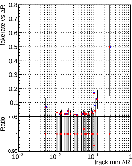
Fake rate vs \Delta R(\text{track, jet}) DQM_TT_ORIGINAL DQM_TT_MODIFIED_layerProcV2_PRVersion
