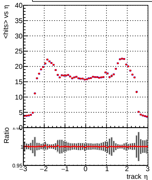
mean hits — DQM_TT_ORIGINAL — DQM_TT_MODIFIED_layerProcV2_PRVersion
