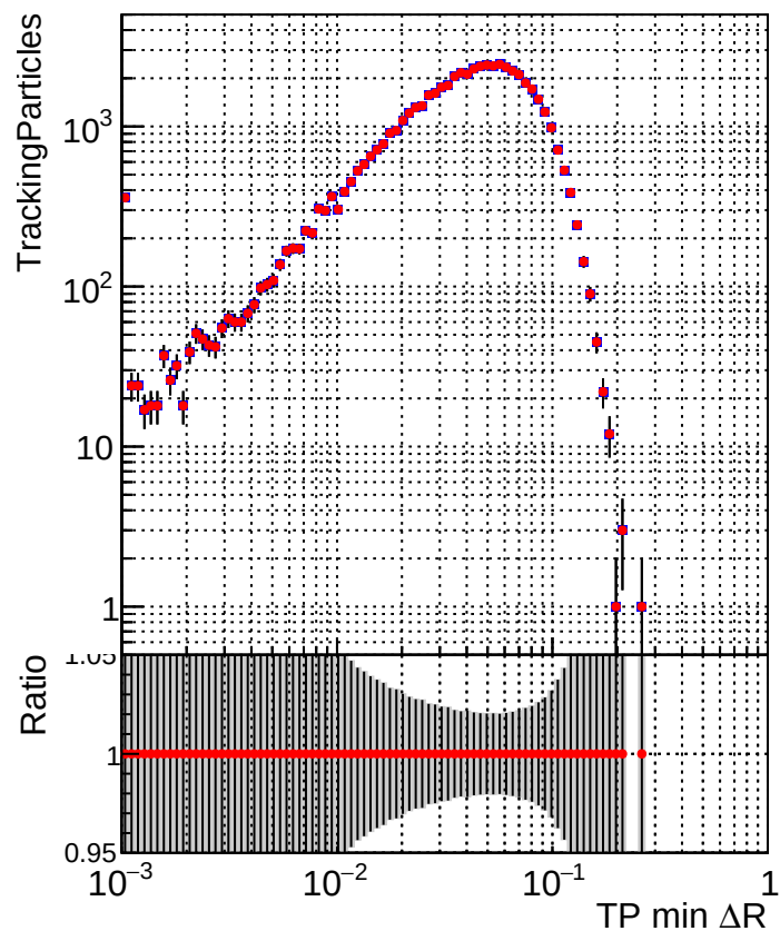
N of simulated tracks vs TP \Delta R (TP, jet) ■ DQM_TT_ORIGINAL — DQM_TT_MODIFIED_layerProcv2_PRVersion
