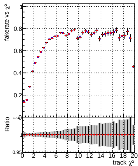
Fake rate vs. Legend: - Blue line with dots: DQM TT ORIGINAL - Red line with dots: DQM TT MODIFIED layerProc2_PRVersion
