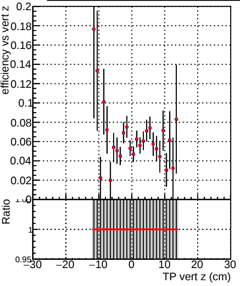
Efficiency vs vertpos Legend: DQM_TT_ORIGINAL DQM_TT_MODIFIED_layerProcv2_PVersion
