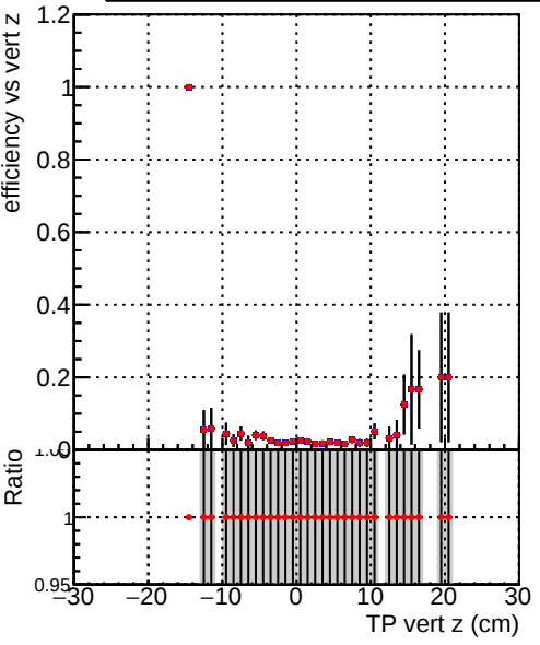
Efficiency vs TP vert z (cm) Legend: DQM_TT_ORIGINAL DQM_TT_MODIFIED_layerProcv2_PVersion
