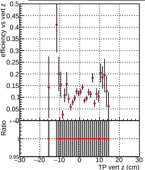
Efficiency vs vert z Legend: DQM_TT_ORIGINAL (grey histogram), DQM_TT_MODIFIED_layerProcv2_PVersion (red stars)
