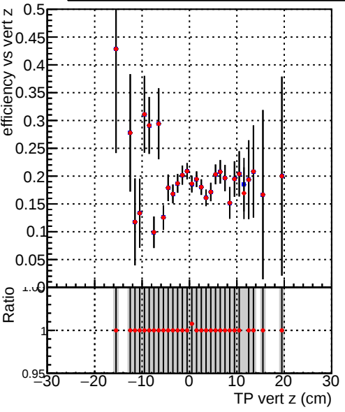
Efficiency vs vert z Legend: DQM_TT_ORIGINAL (blue square), DQM_TT_MODIFIED_layerProcv2_PVersion (red circle)
