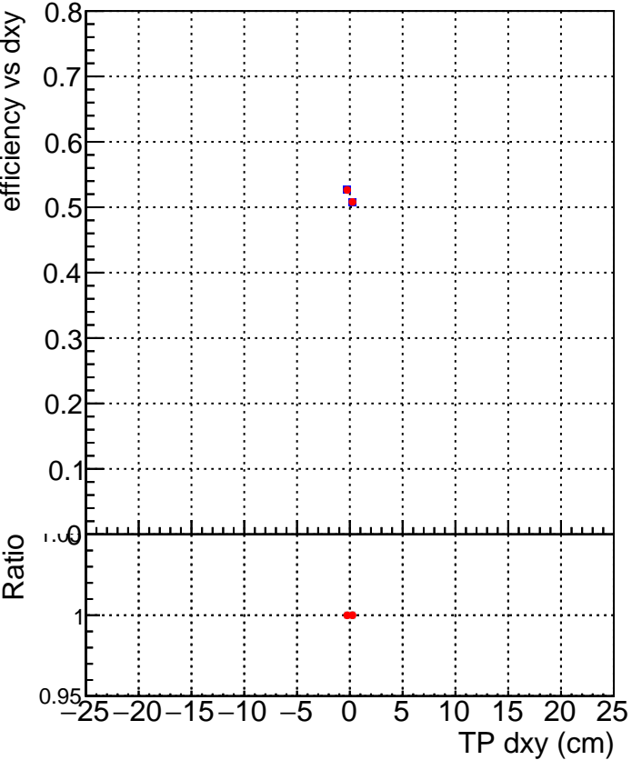
Legend: ■ DQM_TT_ORIGINAL ● DQM_TT_MODIFIED_layerProcv2_PRVersion
