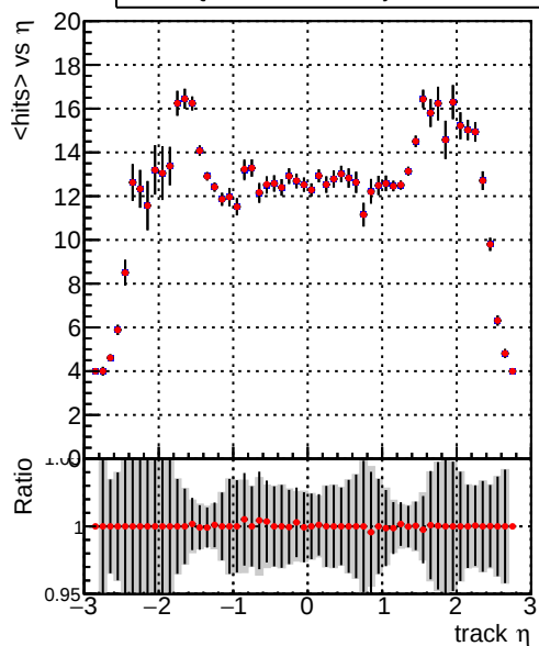
— DQM_TT_ORIGINAL — DQM_TT_MODIFIED_layerProcV2_PRVersion mean hits
