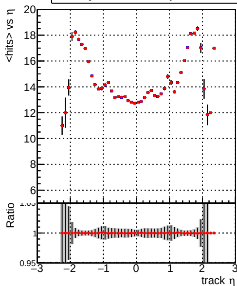
mean hits vs \eta DQM_TT_MODIFIED_layerProcV2_PRVersion
