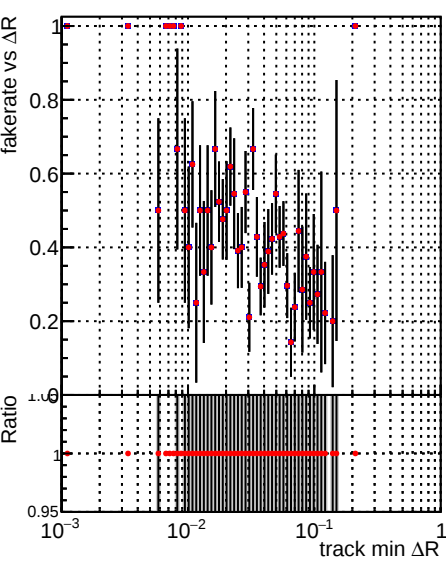
Fake rate vs \Delta R(\text{track, jet}) Legend: —●— DQM_TT_ORIGINAL —●— DQM_TT_MODIFIED_layerProcV2_PRVersion
