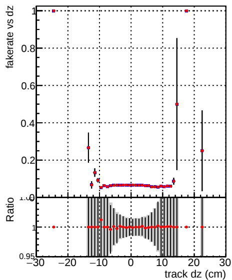
Fake rate vs dz —•— DQM_TT_ORIGINAL —•— DQM_TT_MODIFIED_layerProcV2_PRVersion
