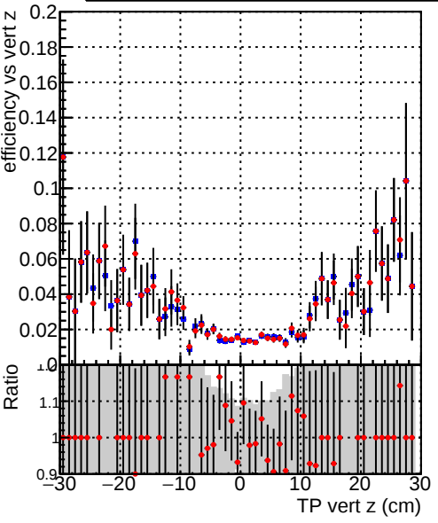
Efficiency vs TP vert z (cm) Legend: DQM_TT_ORIGINAL (blue stars), DQM_TT_MODIFIED_layerProcv2 (red stars)
