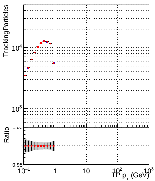
Legend: DQM_TT_ORIGINAL (blue dots), DQM_TT_MODIFIED_layerProcV2 (red dots)
