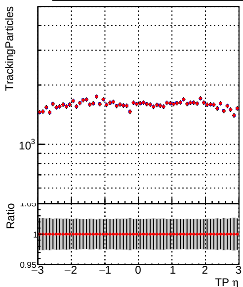
Legend: DQM_TT_ORIGINAL (blue dots), DQM_TT_MODIFIED_layerProcV2 (red dots)
