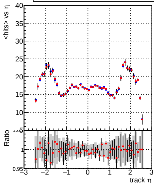
mean hits Legend: DQM_TT_ORIGINAL (blue line), DQM_TT_MODIFIED_layerProc2 (red line)
