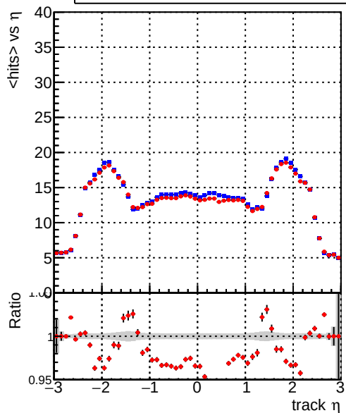
mean hits Legend: DQM_TT_ORIGINAL (blue line), DQM_TT_MODIFIED_layerProcv2 (red line)
