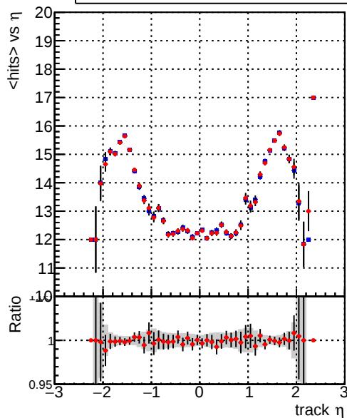
mean hits vs \eta — DQM_TT_ORIGINAL — DQM_TT_MODIFIED_layerProcV2
