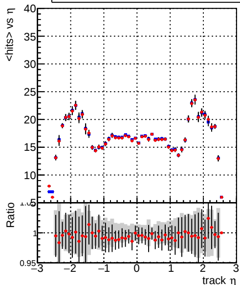
mean hits Legend: DQM_TT_ORIGINAL (blue line), DQM_TT_MODIFIED_layerProcV2 (red line)
