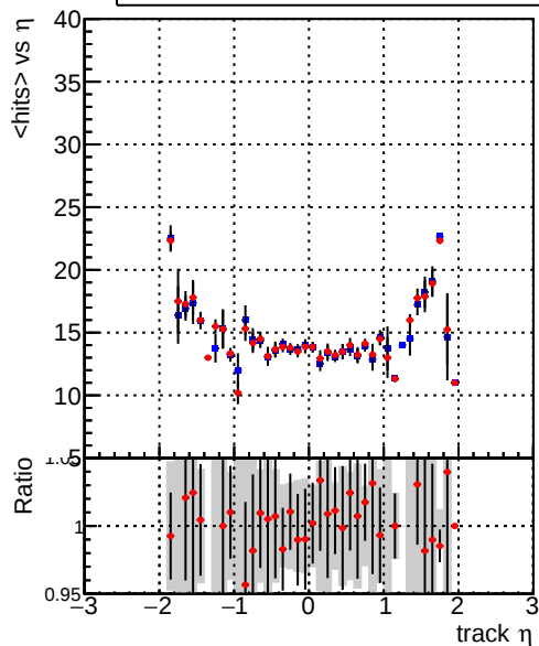
mean hit Legend: DQM_TT_ORIGINAL (blue line), DQM_TT_MODIFIED_layerProcV2 (red line)
