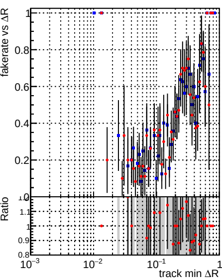
Legend: DQM_TT_ORIGINAL (blue dots), DQM_TT_MODIFIED_layerProcv2 (red dots)
