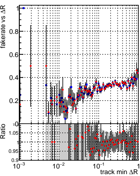
Fake rate vs \Delta R(\text{track, jet}) ■ DQM_TT_ORIGINAL ■ DQM_TT_MODIFIED_layerProcV2
