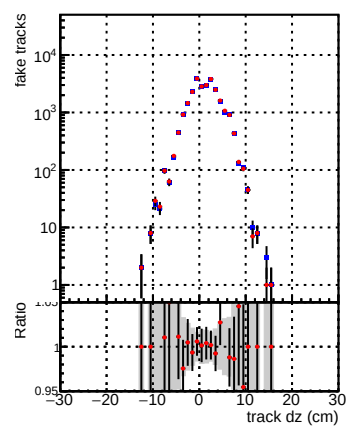
N of fake tracks vs dz
