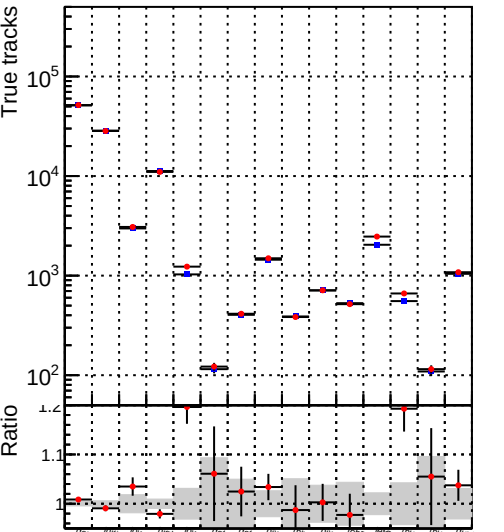
Number of true tracks vs collection
