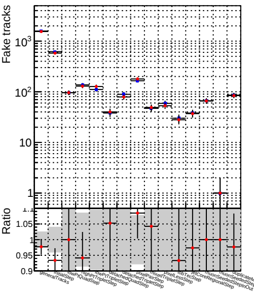
Number —●— DQM_TT__MODIFIED_layerProcv2
