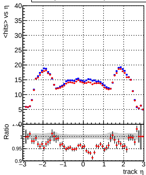
mean hit Legend: DQM_TT_ORIGINAL (Blue line), DQM_TT_MODIFIED_layerProc2 (Red line)
