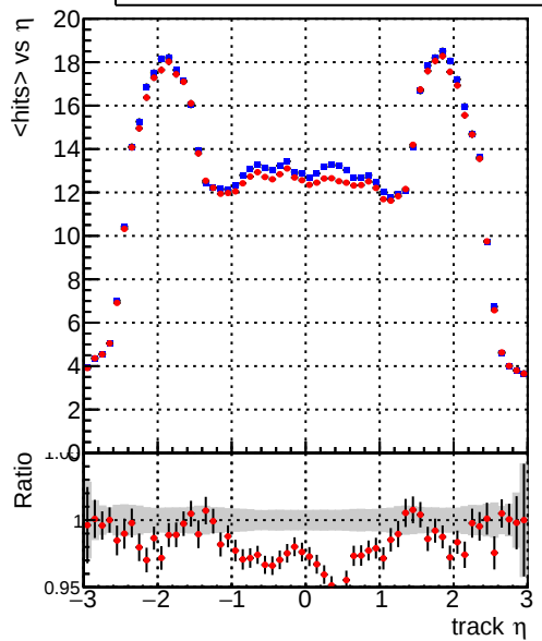
mean hit — DQM_TT_ORIGINAL — DQM_TT_MODIFIED_layerProcV2
