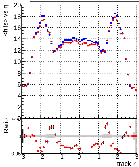
mean hit DQM_TT_ORIGINAL DQM_TT_MODIFIED_layerProcV2
