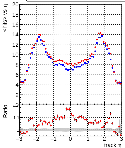
mean hits vs \eta Legend: DQM_TT_ORIGINAL (blue line), DQM_TT_MODIFIED_layerProcv2 (red line)
