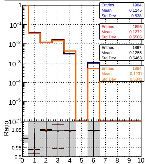
DQM_TT mkFit-DQM_original-0 DQM_TT mkFit-DQM_original-127 DQM_TT mkFit-DQM_mod-127 DQM_TT mkFit-DQM_mod_updated-127 mean hit
