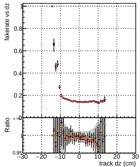
Fake rate vs dz Legend: BQM (black), mkFit-BQM (red), mkFit-BQM-mod (orange), mkFit-BQM-original (blue), mkFit-BQM-mod-updated-127 (grey)
