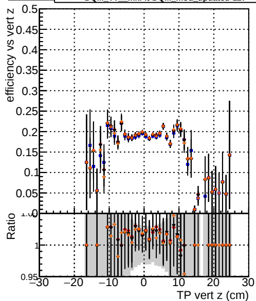
Efficiency vs. sim PV z —●— DOM TT mkFit-DQM original-0 —●— DOM TT mkFit-DQM original-127 —●— DOM TT mkFit-DQM mod-127 —●— DOM TT mkFit-DQM mod updated-127
