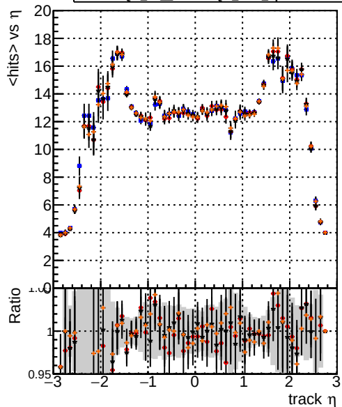
mean hits Legend: DOM TT mkFit-DQM original-0 DOM TT mkFit-DQM original-127 DOM TT mkFit-DQM mod-127 DOM TT mkFit-DQM mod updated-127
