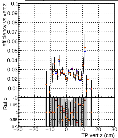
Efficiency vs. TP vert z —●— DOM TT mkFit-DQM original-0 —●— DOM TT mkFit-DQM original-127 —●— DOM TT mkFit-DQM mod-127 —●— DOM TT mkFit-DQM mod updated-127
