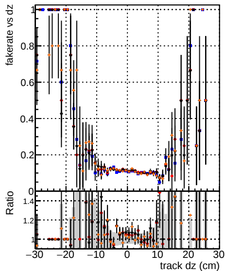
Legend: - \bullet BSM \bullet mkFit BSM original-127 - \circ BSM \circ mkFit BSM mod updated-127
