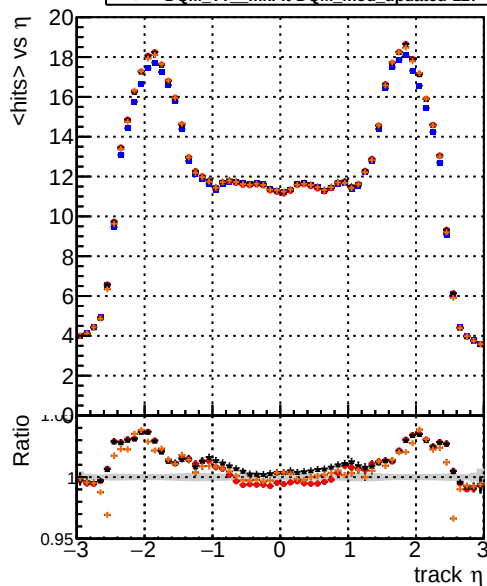
Legend: DQM TT mkFit-DQM original-0 (blue line), DQM TT mkFit-DQM original-127 (red line), DQM TT mkFit-DQM mod-127 (black line), DQM TT mkFit-DQM mod updated-127 (orange line) mean hits
