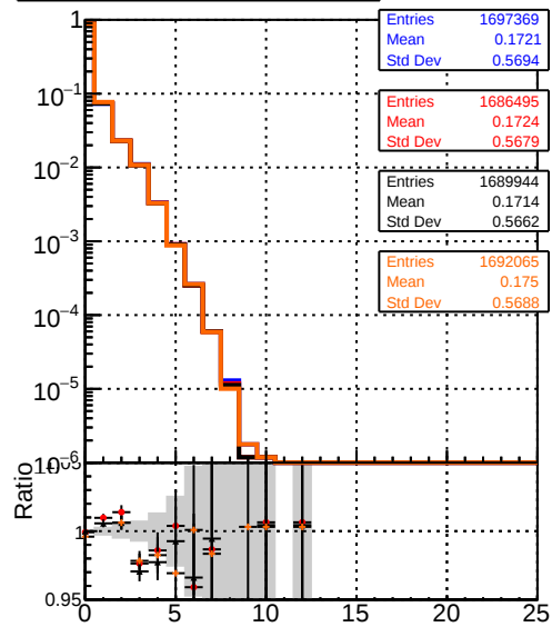
Legend: DQM TT mkFit-DQM original-0 (blue line), DQM TT mkFit-DQM original-127 (red line), DQM TT mkFit-DQM mod-127 (black line), DQM TT mkFit-DQM mod updated-127 (orange line) mean hits
