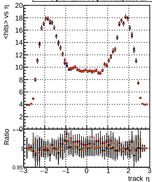
mean hit Legend: DOM TT mkFit-DQM original-0 DOM TT mkFit-DQM original-127 DOM TT mkFit-DQM mod-127 DOM TT mkFit-DQM mod updated-127
