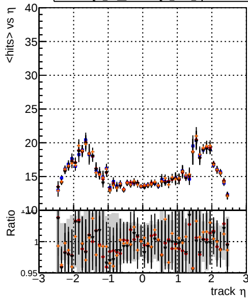
mean hit Legend: DQM_TT mkFit-DQM_original-0 DQM_TT mkFit-DQM_original-127 DQM_TT mkFit-DQM_mod-127 DQM_TT mkFit-DQM_mod_updated-127
