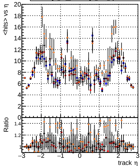
mean hit Legend: DOM_TT mkFit-DQM_original-0 DOM_TT mkFit-DQM_original-127 DOM_TT mkFit-DQM_mod-127 DOM_TT mkFit-DQM_mod_updated-127
